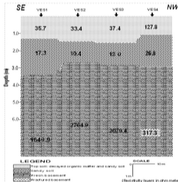
Figure 14: Geoelectric section beneath VES 1, 2, 3 and 4
