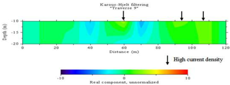
Figure 10: Karous-Hjelt current density plots for VLF-em profile 6
