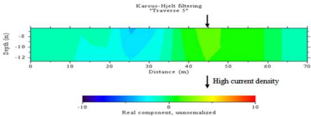
Figure 7: Karous-Hjelt current density plots for VLF-em profile 3
