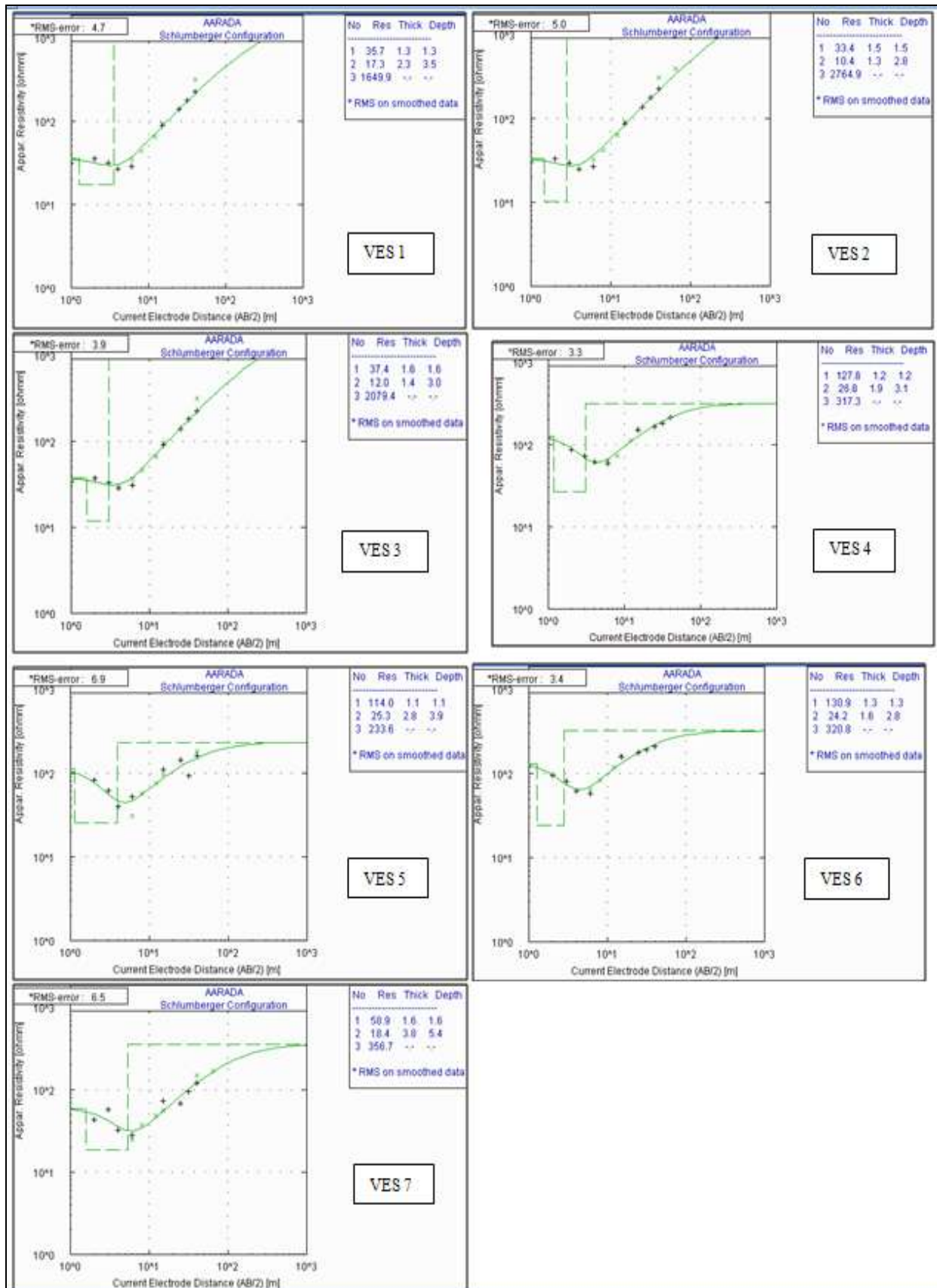
Figure 13: The model curves for VES 1 to VES 7
