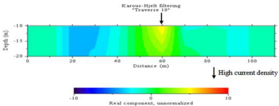
Figure 11: Karous-Hjelt current density plots for VLF-em profile 7
