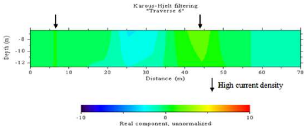
Figure 8: Karous-Hjelt current density plots for VLF-em profile 4
