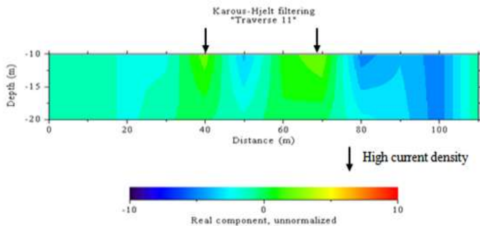
Figure 12: Karous-Hjelt current density plots for VLF-em profile 8
