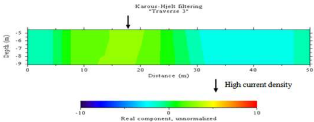
Figure 5: Karous-Hjelt current density plots for VLF-em profile 1
