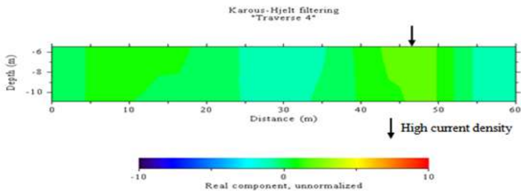
Figure 6: Karous-Hjelt current density plots for VLF-em profile 2
