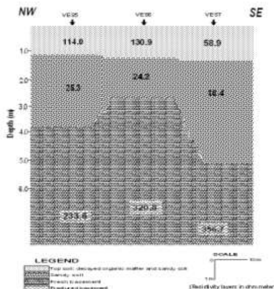
Figure 15: Geoelectric section beneath VES 5, 6 and 7
