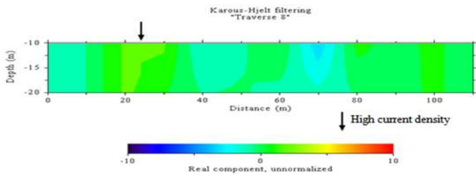
Figure 9: Karous-Hjelt current density plots for VLF-em profile 5
