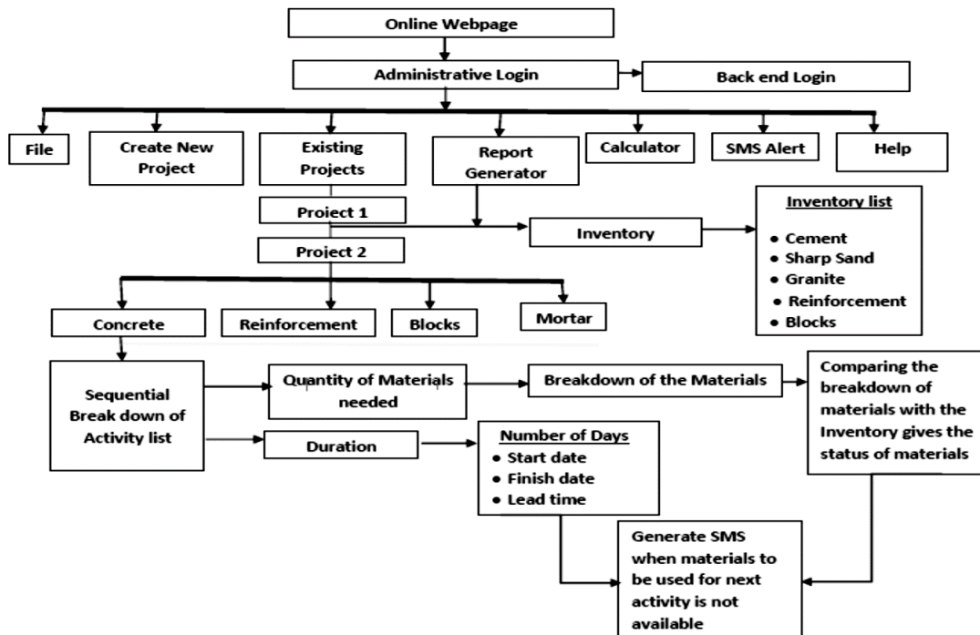
Figure 4. System Block Diagram of the WB-MPC
