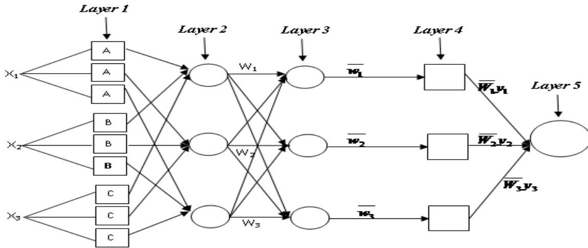
Fig.4. Three inputs ANFIS Model for Handover Process
