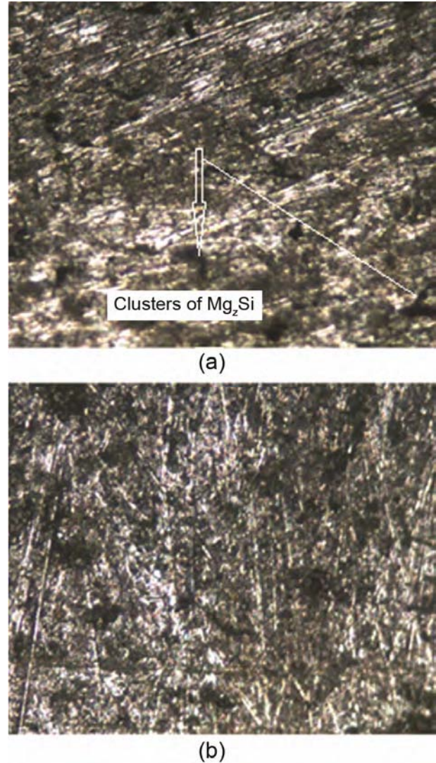
Fig. 9 – Micrograph of extruded samples for die of 75° entry angle using (a) mild steel and (b) tool steel
