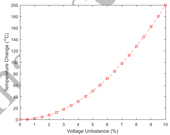
Figure 8. Temperature rise with increasing percentage voltage unbalance
