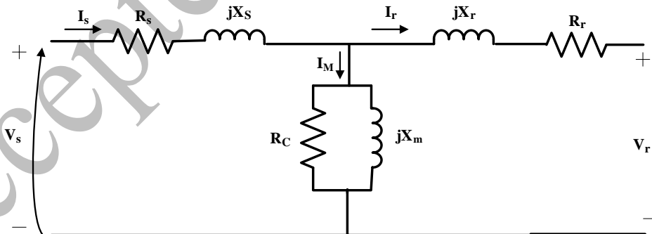
Figure 3. Equivalent T-circuit of a 3-phase induction
