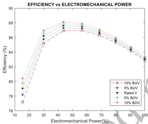
Figure 5. A plot of efficiency against electromechanical power
