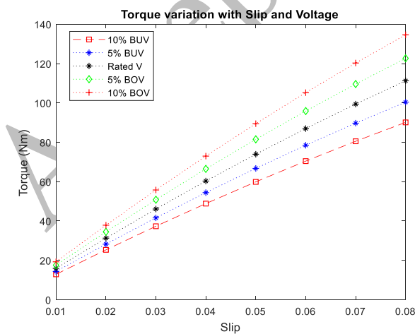
Figure 6. Motor output torque variation
