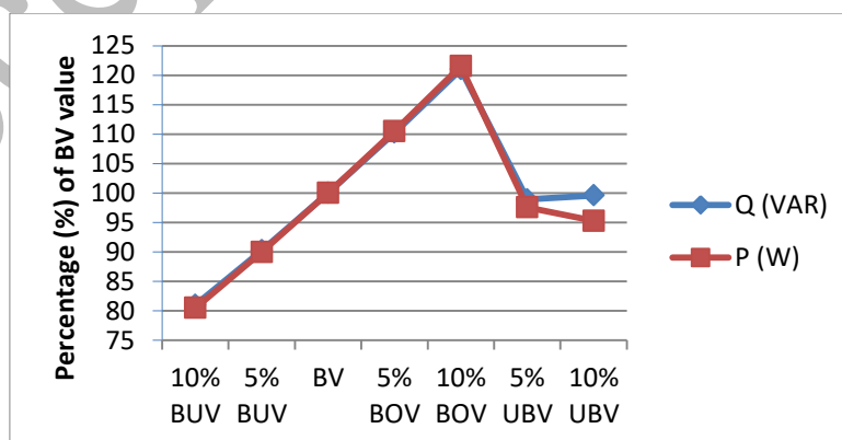
Figure 10. Real and reactive input power for the voltage variations
