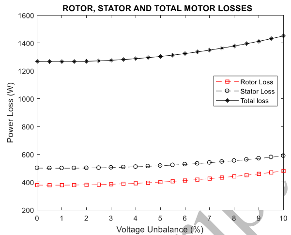
Figure 7. Rotor, Stator and Total loss with increasing unbalance
