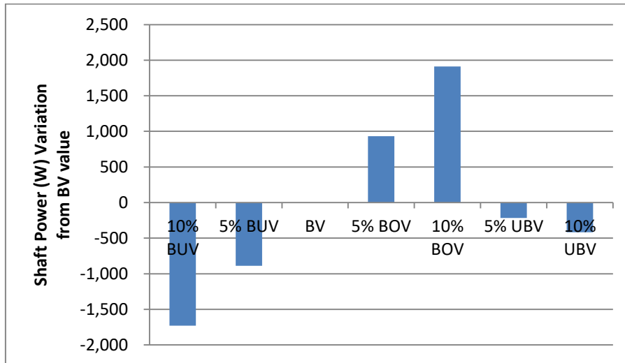
Figure 11. Shaft power variation with respect to the BV value
