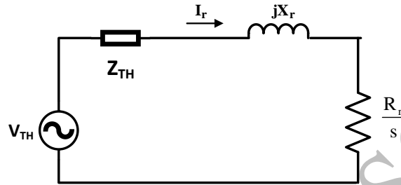
Figure 2. Thevenin equivalent of a 3-phase induction motor
