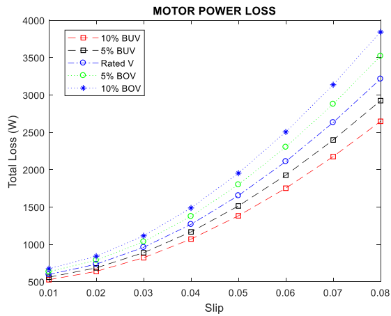
Figure 4. Total energy loss in the motor
