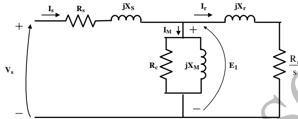
Figure 1. The Per Phase Equivalent Circuit of a 3-phase induction motor
