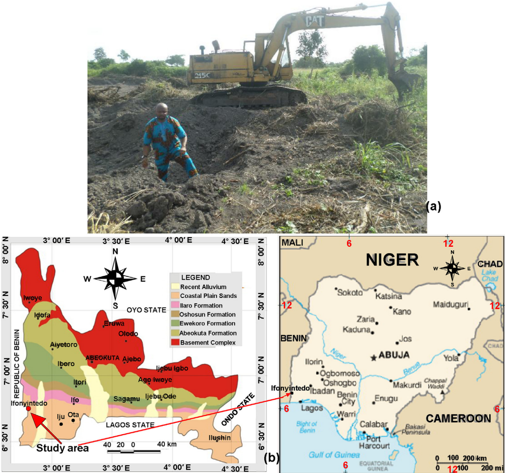
Fig. 1. (a) Kaolin mining in Ifonyintedo; (b) Geological domains of Ogun state, Nigeria revealing Ifonyintedo.
