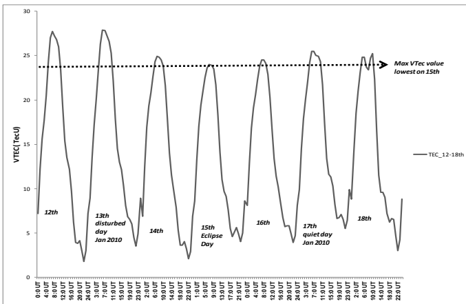
Figure 3a: Daily VTEC variations 3-days before and 3-days after Solar Eclipse at UKM
