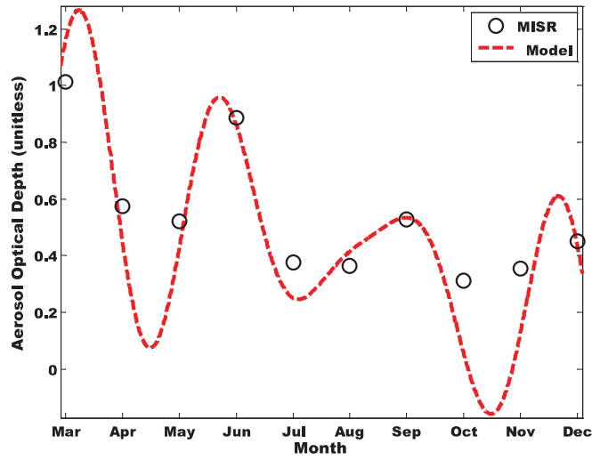
FIGURE 3. AOD pattern for Kano 2000
