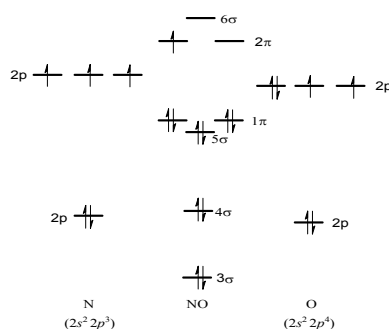
Figure 1. Molecular orbital energy level diagram for NO [4]
