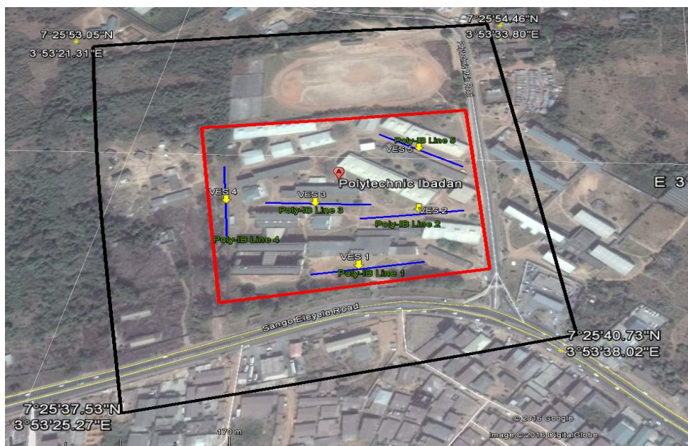
Fig. 2: Satellite imagery map of the study site in Ibadan indicating the 2D resistivity profile lines (blue) and VES points (yellow arrows)
