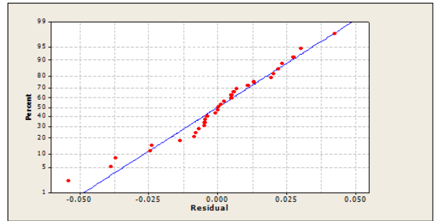
Figure 2: Normal Percent plot of residuals for tool wear.
