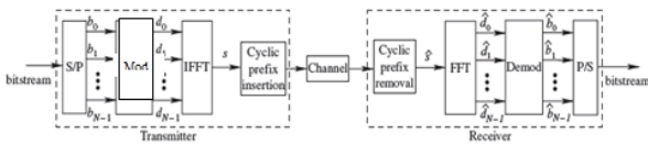
Fig. 2. Block Diagram of an OFDM system [7]
