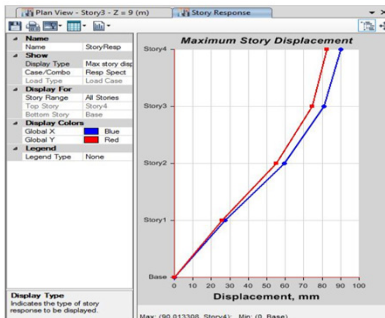
Fig. 4. Storey Displacements
