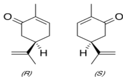
Fig. 9 Structure of Carvone
