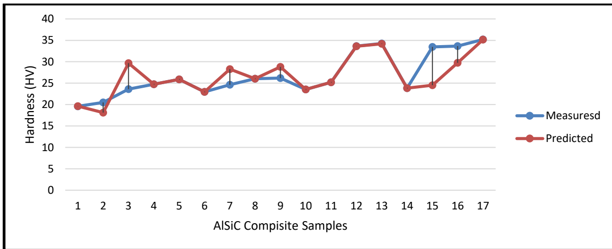
Fig. 12 Measured and predicted hardness of AMC Composites
