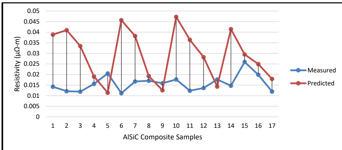
Fig. 14 Measured and predicted resistivity of AMC Composites
