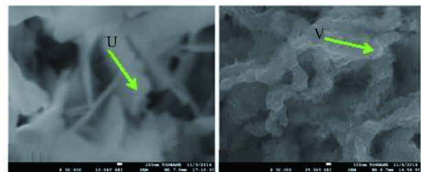
Fig. 6 SEM/EDS of (a) and (c) Zn-TiO 2 -WO 3 -8g-1.0A (b) and (d) Zn-TiO 2 -WO 3 -15g-1.5A coated mild steel showing the internal morphology of the coatings at the nanolevel- 100 nm ('U' and 'V' are Zn-TiO 2 -WO 3 -rich portions)
