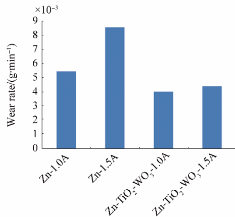
Fig. 14 Variation of wear rate of Zn-TiO 2 -WO 3 and Zn coated steel with time
