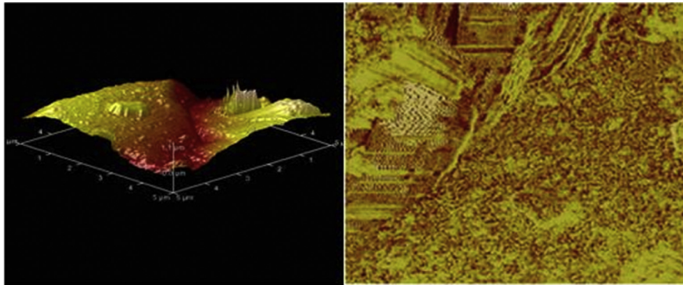
Fig. 3. AFM of Zn–8ZnO–16SiO 2 deposited at 1 A/cm 2 for 15 min.
