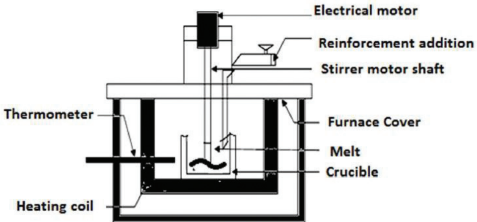
Figure 12. Schematic view of stir casting setup [7].
