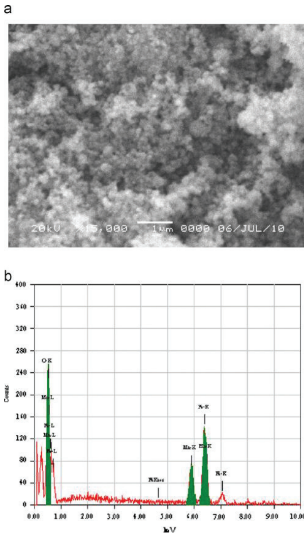
Figure 4. (a) SEM micrograph and (b) EDX of manganese ferrite ( Mn-Fe_2O_4 ) powder prepared by hydrothermal route [15].
