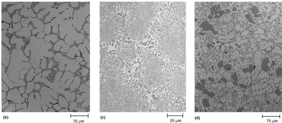
Figure 5. Commercial cast aluminum-silicon alloys. (a) Al-Si equilibrium diagram; (b) microstructure of hypoeutectic alloy (1.65–12.6 wt.% Si) 150; (c) microstructure of eutectic alloys (12.6% Si) 400; and (d) microstructure of hypereutectic alloy (>12.6% Si) 150 [16].
