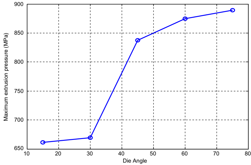
Fig. 3. Effect of maximum extrusion pressure against die angle.
