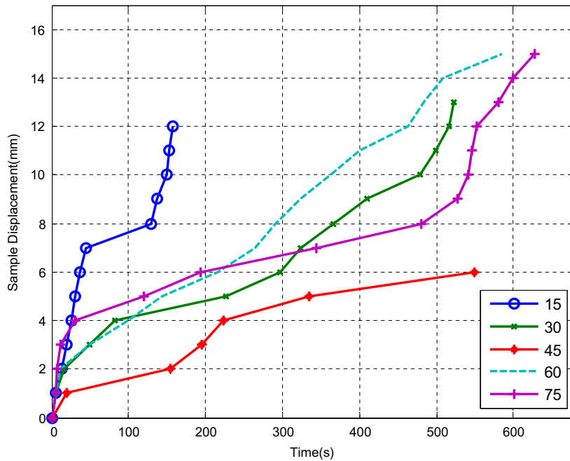
Fig. 4. Variation of sample displacement with time.
