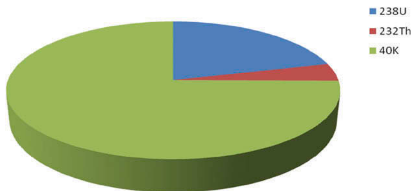
Figure 2. Mean activities in mining area.
