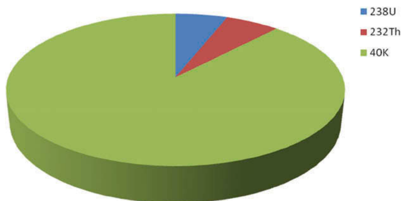
Figure 3. Mean activities in living area.
