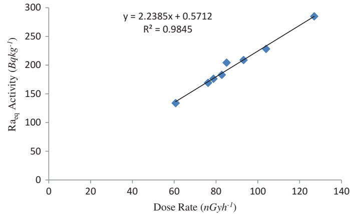
Figure 4. Correlation of radium equivalent with dose rate in mining area.
