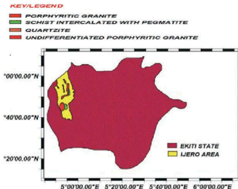
Figure 1. Geological map of Ijero Ekiti (Modified after Ale, Dada, & Adewumi, 2014).
