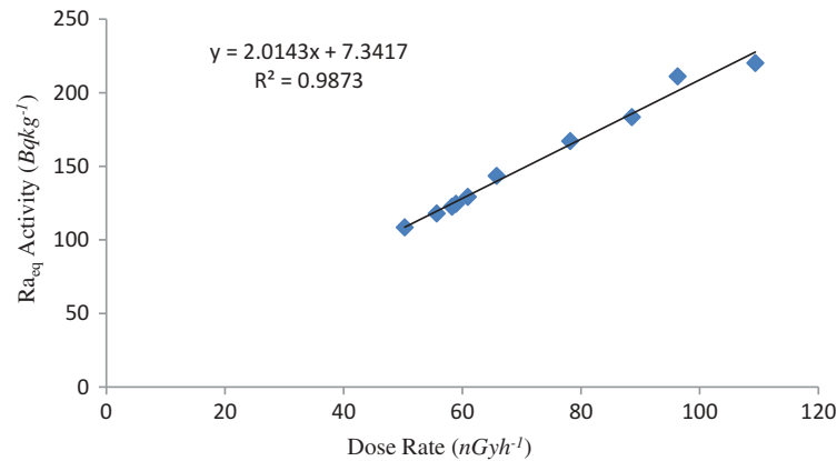
Figure 5. Correlation of radium equivalent with dose rate in living area.
