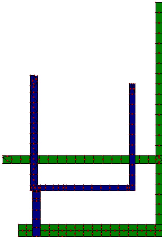
Figure 9. Current distribution of the proposed antenna.
