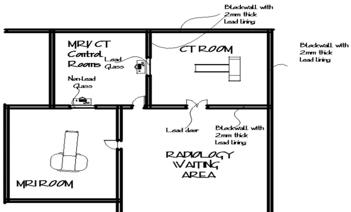
Figure 4: Sketch showing Floor plan of CT and MRI room sharing one control room.
