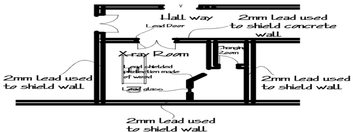
Figure 5: Sketch showing the Floor Plan x-ray room.
