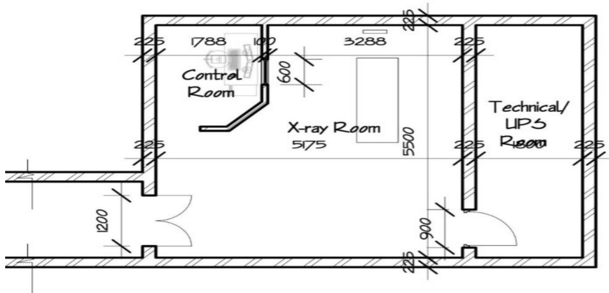
Figure 10: Sketch showing the x-ray room; Source: Author's field Study (2019)
