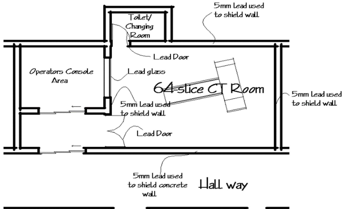
Figure 8: Sketch showing the 64 slice computed tomography room.
