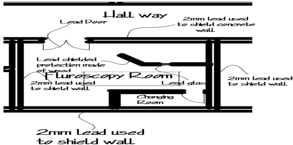
Figure 6: Sketch showing the floor plan of fluoroscopy room.
