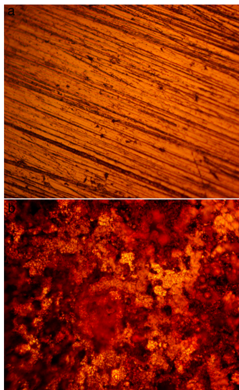
Fig. 4 – Optical microscopic image of HCS at mag. 40× (a) before corrosion, (b) after corrosion in 0% LCN/1 M HCl.
