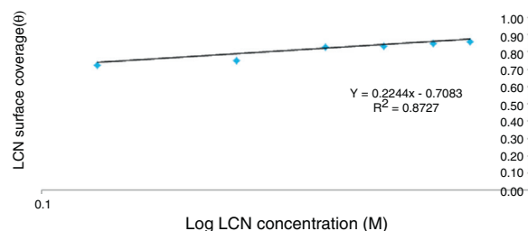
Fig. 8 – Freundlich isotherm plot of log LCN concentration vs log surface coverage.
