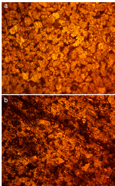
Fig. 5 – Optical microscopic image of HCS at mag. 40× (a) after corrosion in 0.91% LCN/1 M HCl, (b) after corrosion in 5.63% LCN/1M HCl.
