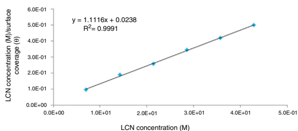
Fig. 6 – Langmuir plot of C_{LCN}/\theta versus LCN concentration in 1 M HCl.
