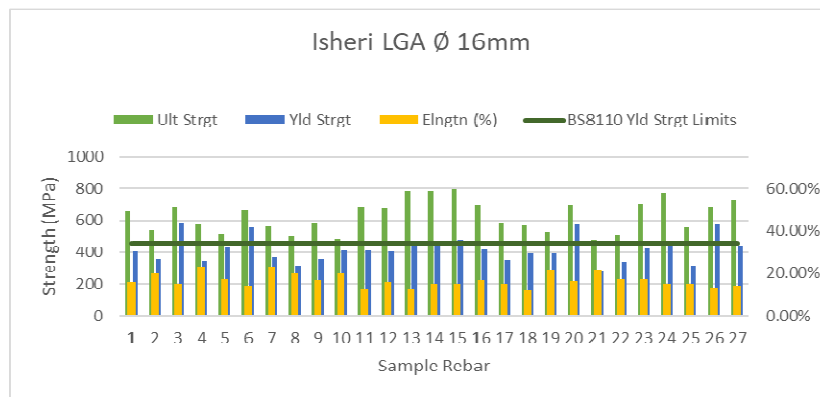
Figure 4. Rebar Ultimate strength, Yielding Strengths and Elongations for Isheri LGA's samples
