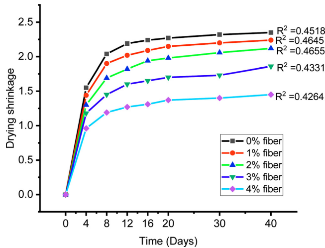
Fig. 12. Drying Shrinkage of Concrete containing Human Hair.
