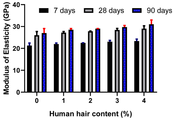
Fig. 11. Modulus of Elasticity of Concrete containing Human Hair.
