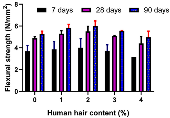
Fig. 10. Flexural Strength of Concrete.
