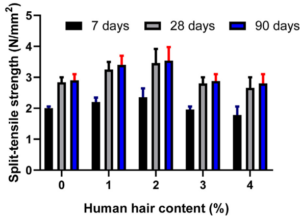
Fig. 9. Indirect Tensile Strength.
