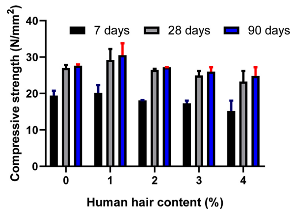
Fig. 8. Compressive Strength of Concrete.
