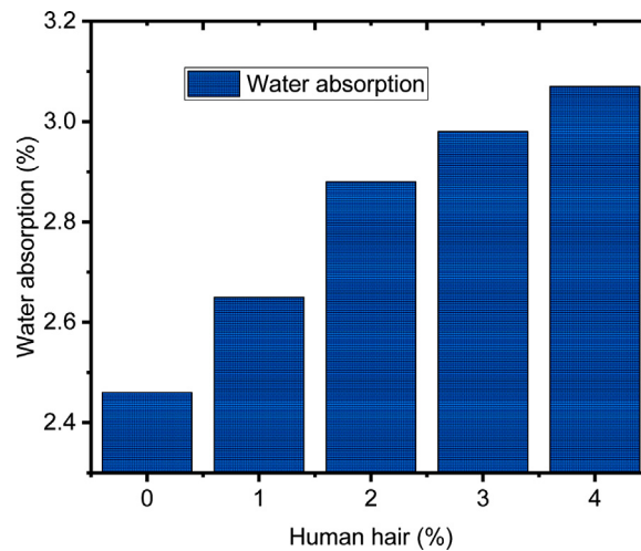
Fig. 7. Water Absorption of Concrete.
