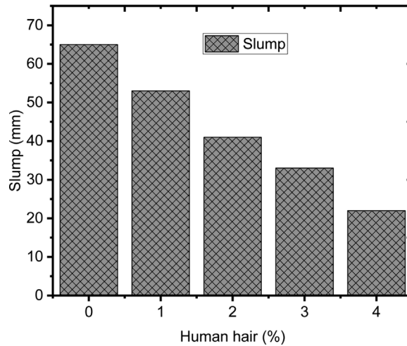
Fig. 5. Slump Test of Concrete.
