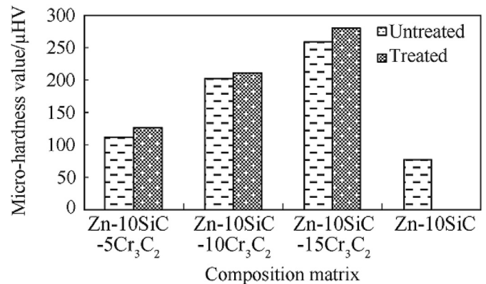
Fig. 4. Hardness property of Zn-10SiC-15 \text{Cr}_3\text{C}_2 coatings before and after heat treatment.
