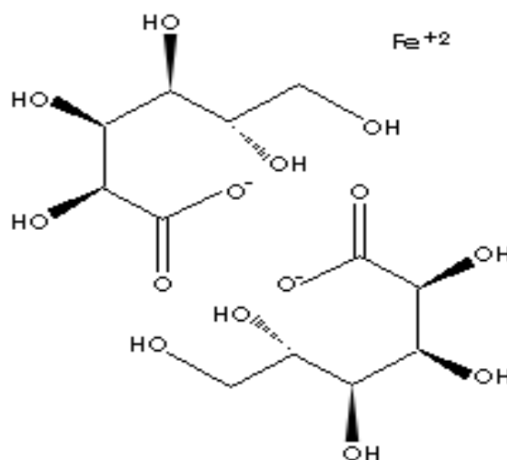
Figure 1. Molecular structure of Ferrous Gluconate
