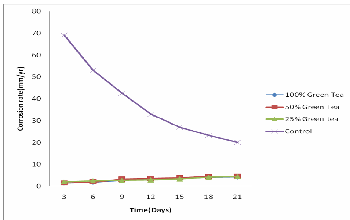
Figure 2: Variation of corrosion rate with exposure time for the mild steel specimen immersed in 0.2M H 2 SO 4 and addition of different concentrations of green tea extract
