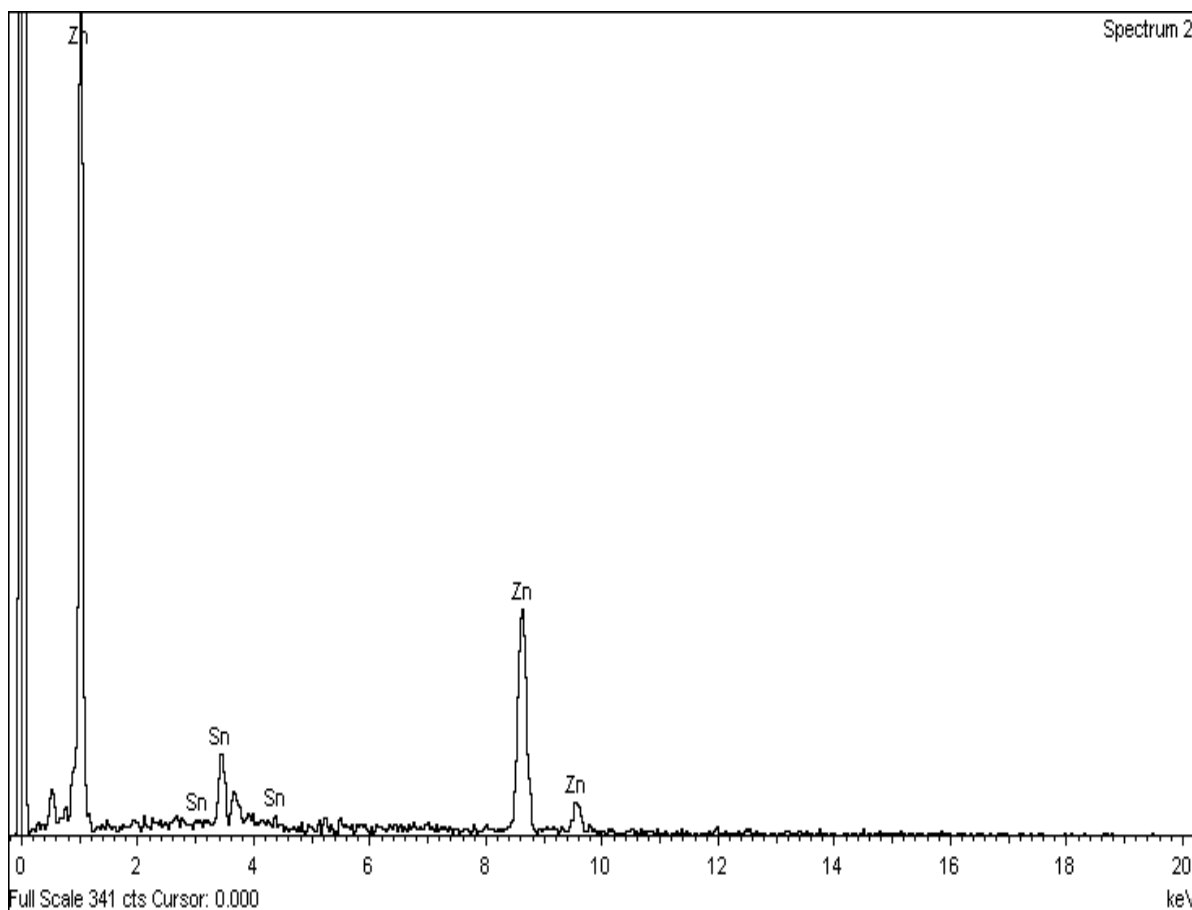
Figure 7. EDS analysis of the plated surface of sample in Fig.3 (iv)
