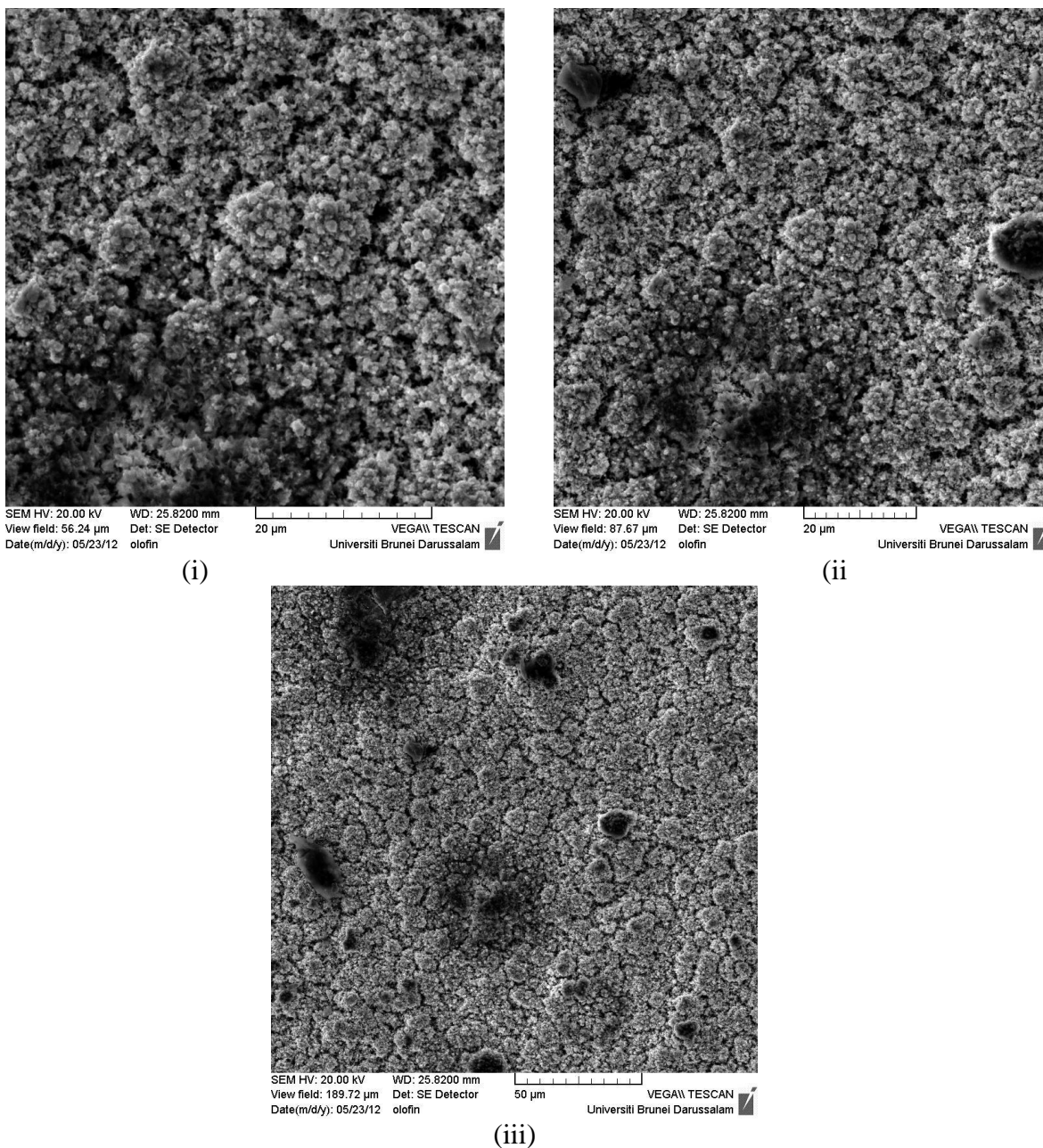
Figure 4. SEM micrographs of steel surface after zinc electrodeposition with 5ml /50ml of acid chloride solution at 15 min. (i) x5000; (ii) and (iii) are x3000, and x1000 magnification respectively
