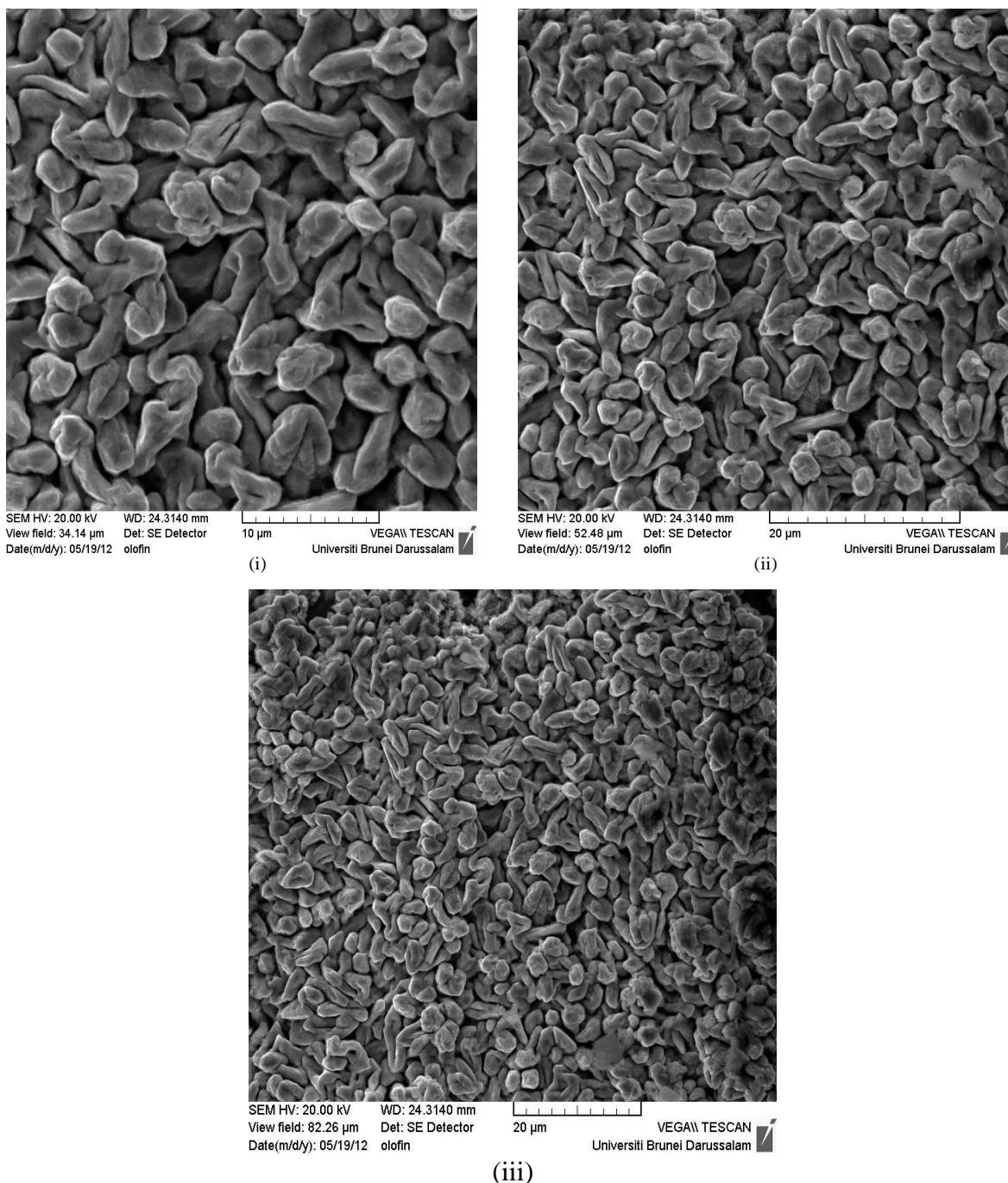
Figure 5. SEM micrographs of steel surface after zinc electrodeposition with 6ml /50ml of acid chloride solution at 15 min. (i) x8000; (ii) and (iii) are x5000, and x3000 magnification respectively
