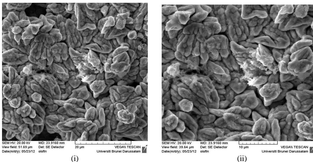
Figure 6. SEM micrographs of steel surface after zinc electrodeposition with 6ml /50ml of acid chloride solution at 18 min. (i) x5000 and (ii) x7000 (iii) magnification respectively
