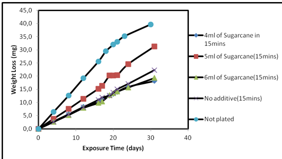
Figure 8. Variation of weight loss with exposure time for the zinc electrodeposited mild steel - sample in seawater. (Variable additive concentrations and 15 minutes plating time)
