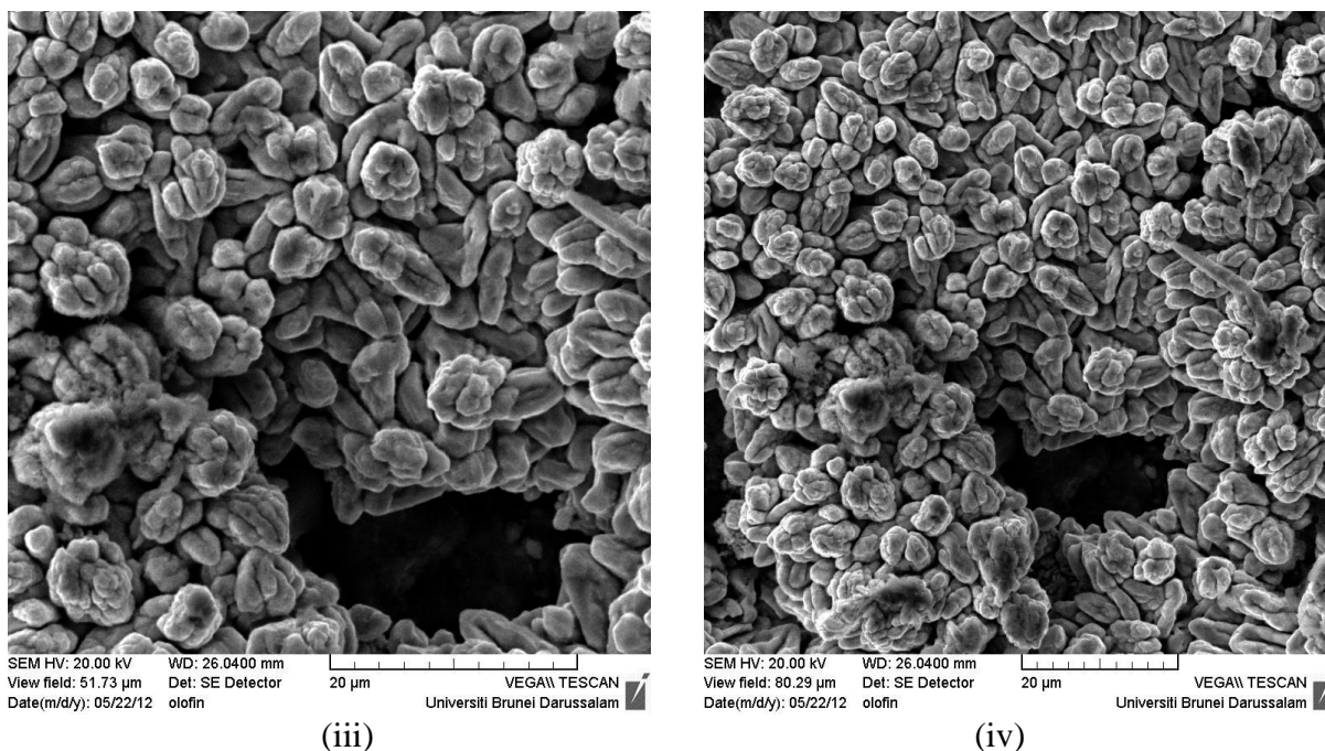
Figure 2. SEM micrographs of mild steel test sample: (i) Before zinc electrodeposition (ii) Plating without additive; (iii) and (iv), plating with 4ml /50ml of acid chloride solution at 15 min. and at the Magnification of: x5000 and x3000 respectively.
