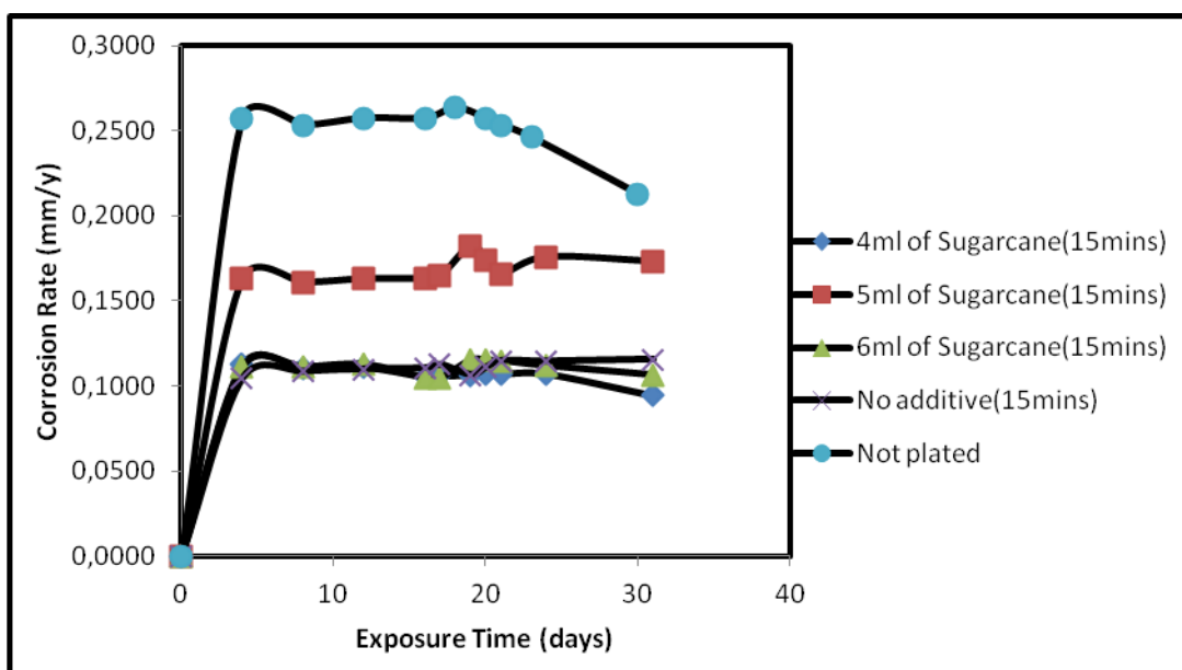
Figure 9. Variation of corrosion rate with exposure time for the zinc plated mild steel samples in seawater. (Variable additive concentrations and 15 minutes plating time)
