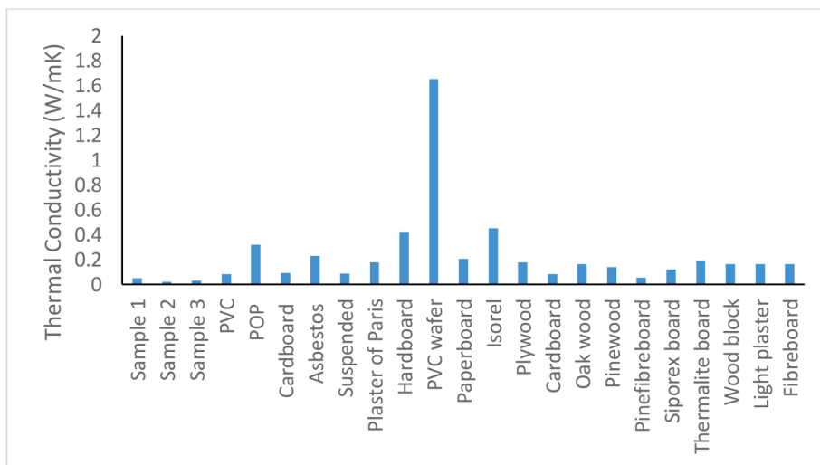
Fig. 8. Thermal conductivity of developed and existing ceiling samples.
