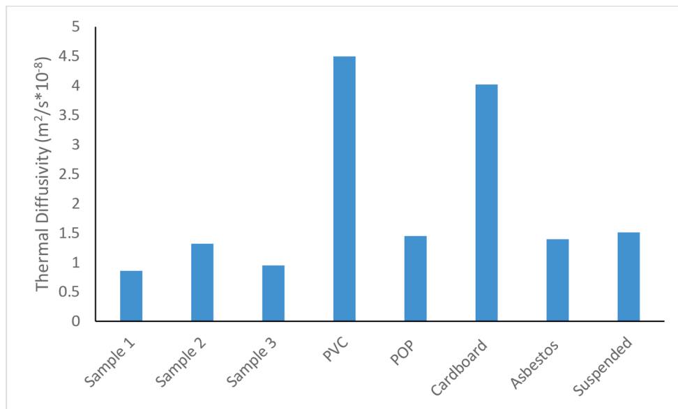
Fig. 9. Thermal diffusivity of developed and existing ceiling samples.
