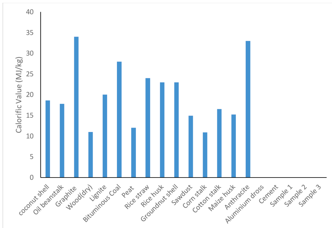
Fig. 10. Calorific value of starting materials and developed ceilings.
