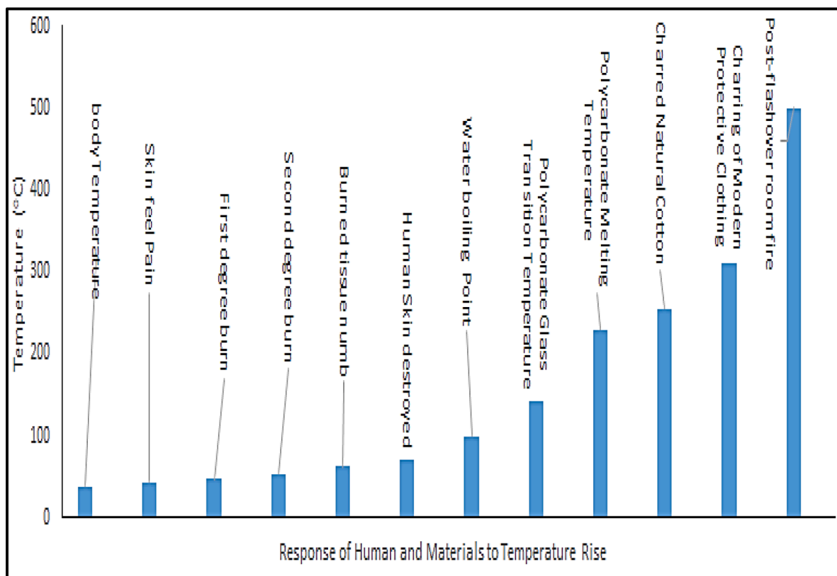
Fig. 6. Human and material response to temperature [74].
