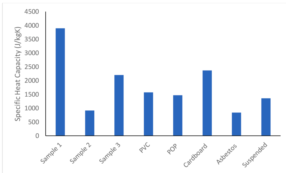
Fig. 7. Specific heat capacity of developed samples and existing ceiling Samples.
