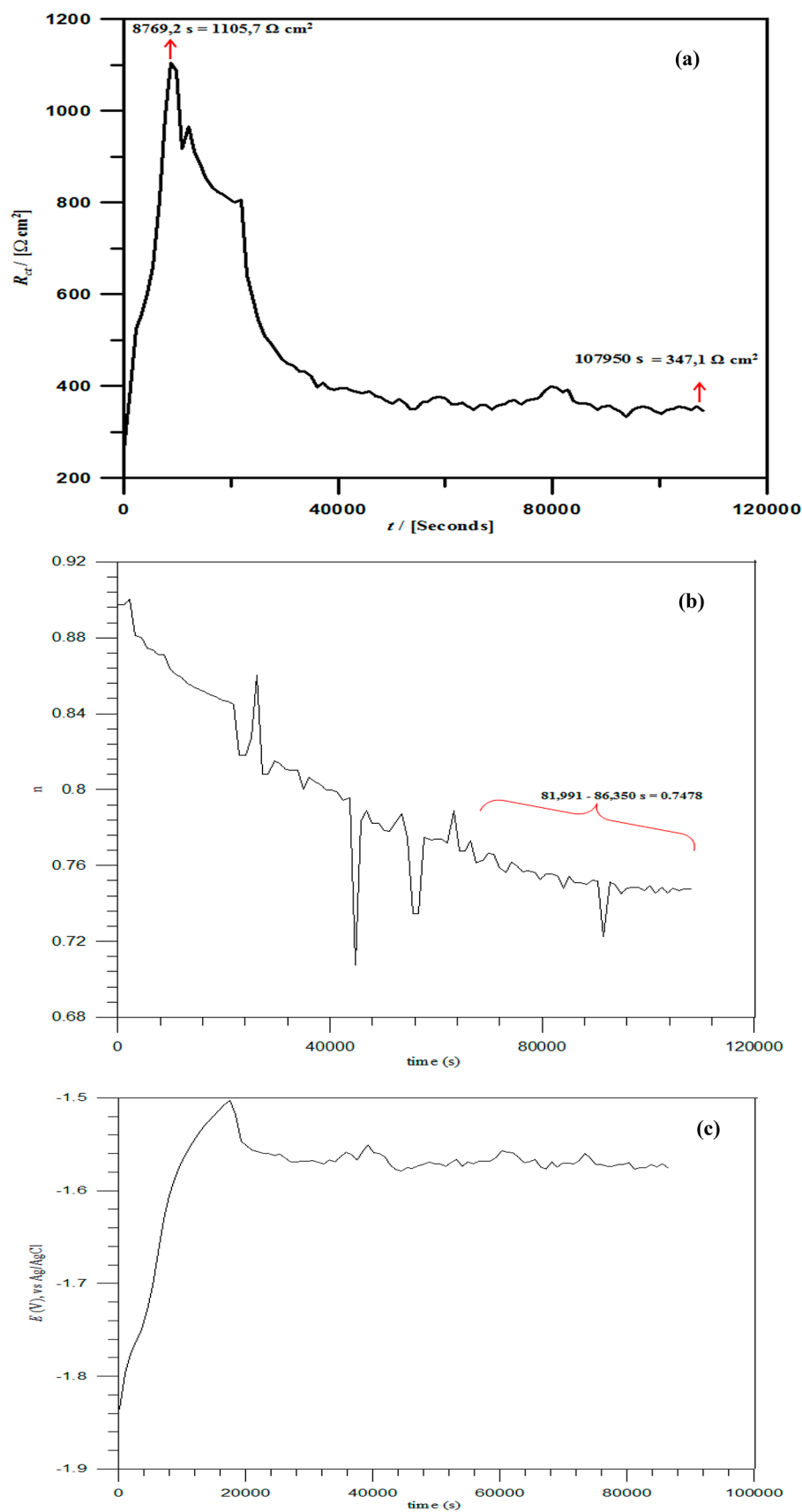
Figure 4. Plot showing the variation of (a) charge-transfer resistance, (b) the n parameter, and (c) the corrosion potential for the AZ91 Mg alloy in simulated body fluid with immersion time.
