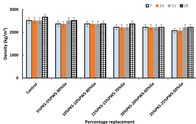
Fig. 7. Density of concrete produced with granite, PKS and PWS for mix 1:1.5:3.
