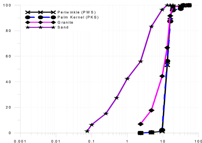
Fig. 5. Particle size distributions for the River Sand (RD) granite (Ge), periwinkle shells (PWS), and palm kernel shells (PKS).
