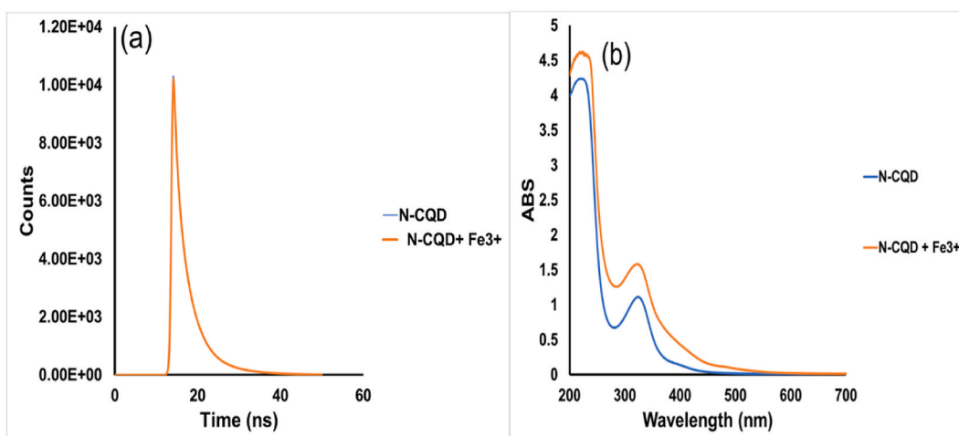
Fig. 6. (a) Fluorescence lifetime decay curve of N -CQDs in the absence and presence of \text{Fe}^{3+} (b) UV-Vis spectra of N -CQDs in the absence and presence of \text{Fe}^{3+} .
