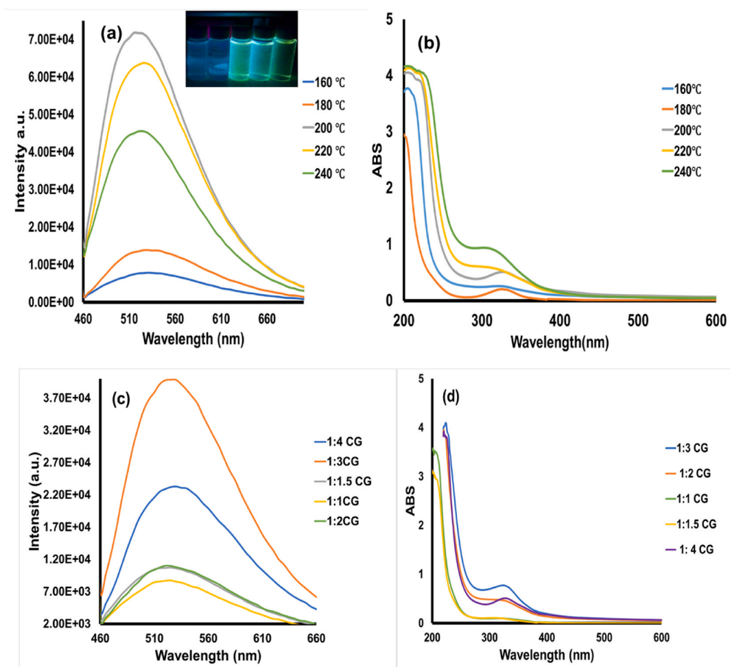
Fig. 1. (a) PL spectra of the as -synthesised N -CQDs at the different reaction temperatures, inset: digital photograph of the corresponding N -CQDs solution under UV-lamp ( \lambda = 365 \text{ nm} ) (b) Absorption spectra of N -CQDs at the different reaction temperatures, (c) PL spectra of the as -synthesised N -CQDs at different citric acid: glutamine precursor molar ratio at 200 °C and (d) Absorption spectra of the as -synthesised N -CQDs at different citric acid: glutamine precursor molar ratio at 200 °C.
