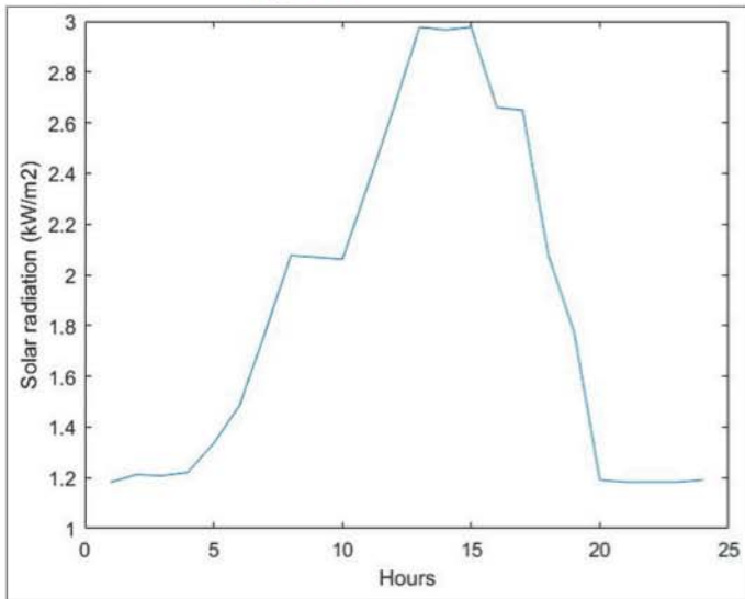
Figure 4: Solar radiation
