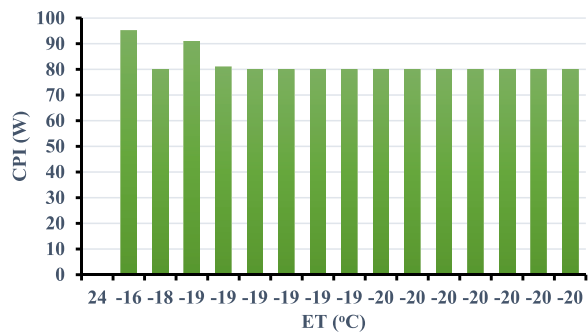
Fig. 8. Effect of power input on ET at 24 °C ambient temperature.
