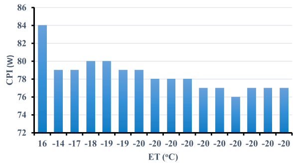
Fig. 6. Effect of power input on ET at 16 °C ambient temperature.
