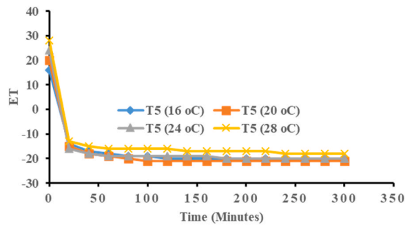
Fig. 5. Pull down time at four different cases of ambient temperature.
