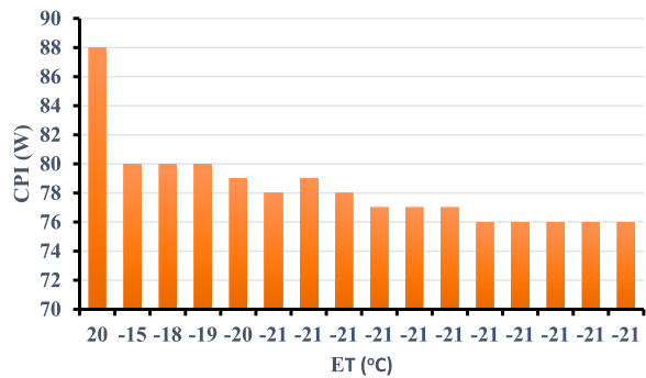
Fig. 7. Effect of power input on ET at 20 °C ambient temperature.
