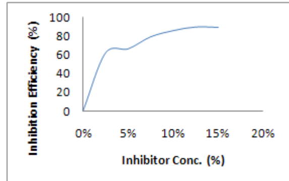
Fig. 5 Percentage inhibition efficiency of DMEA at varying concentrations from weight loss.
