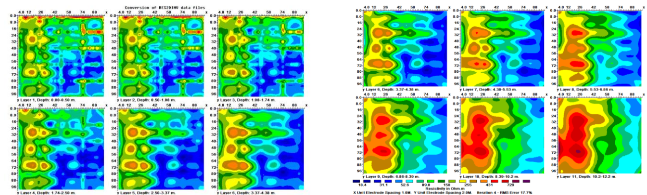
Figure 3: Horizontal depth slices of the 3D inverse model obtained from the orthogonal 2D profiles (field data).
