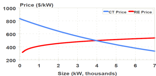
Fig 2: Capital Cost Comparison of Small Gas Turbine Products with Reciprocating Engine Products
