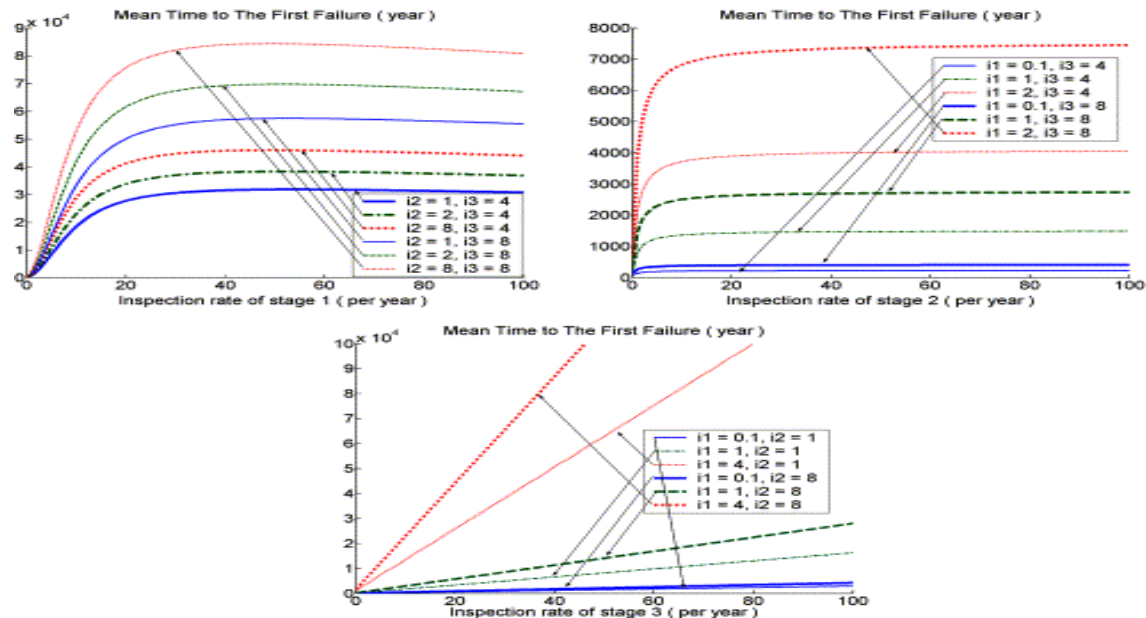
Fig. 4.1a -4.1c The relationship between inspection rate and MTTFF when stage 1 is represented by three sub-units.
