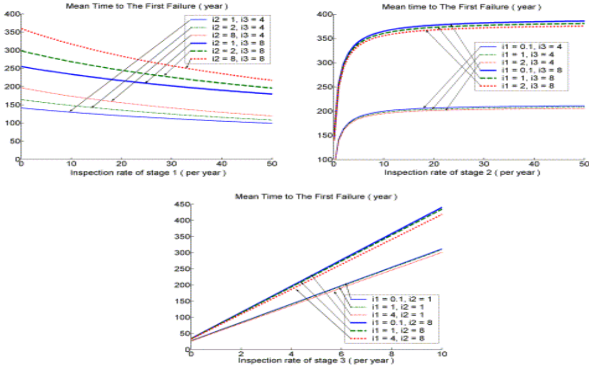
Fig. 4a. – 4c the relationship between inspection rate and MTTFF
