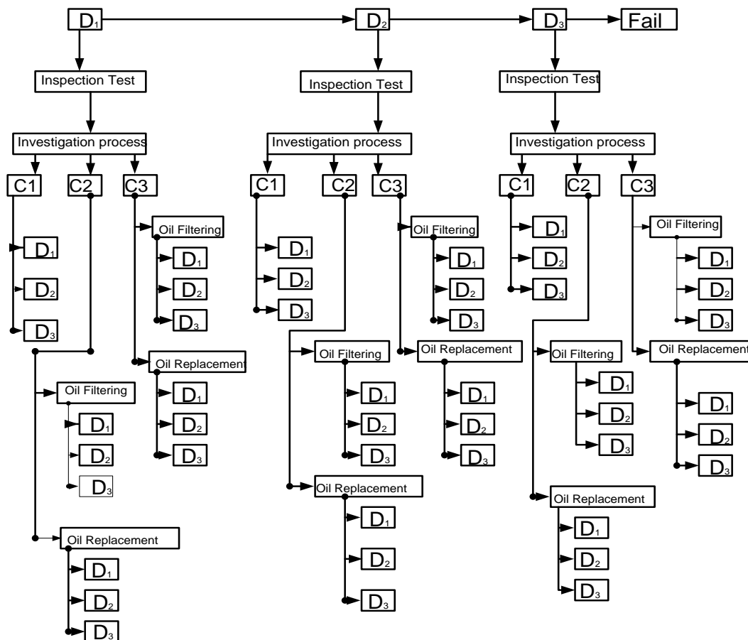
Figure 3.1 Transformer Maintenance Model
