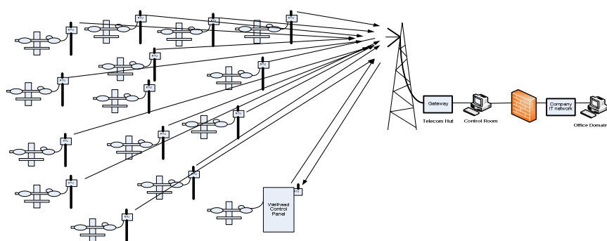
Figure 1: Typical Digital Oilfield communication architecture.
