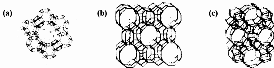
Fig. 4: Schematic representation of (a) sodalite units in \bar{Y} zeolite, (b) mordenite framework structure (c) characteristic framework structure of ZSM-5 zeolite showing channel network (Baerlocher et al., 2007).
