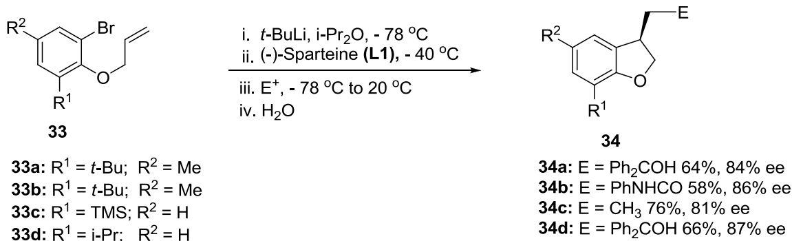
Scheme (10). Intramolecular carbolithiated synthesis of 2,3-dihydrobenzofurans 34 .
