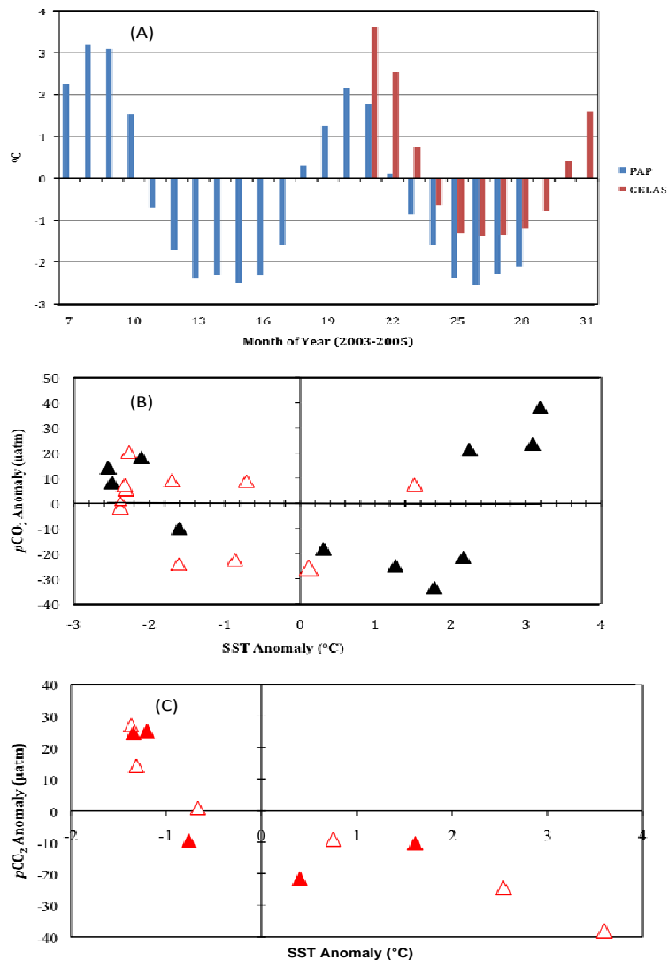
Figure 3. (a) Monthly SST anomalies (°C) at the K1 Central Labrador Sea (CELAS) and Porcupine Abyssal Plain (PAP) sites between July 2003 – July 2005, (b) Monthly anomalies of p\text{CO}_2 against SST monthly anomalies at the PAP site for fall/winter period (transparent red triangles) and the spring/summer period (black triangles), (c) Monthly anomalies of p\text{CO}_2 against SST at the K1 CELAS site for the fall/winter period (transparent red triangles) and spring/summer period (red triangles).
