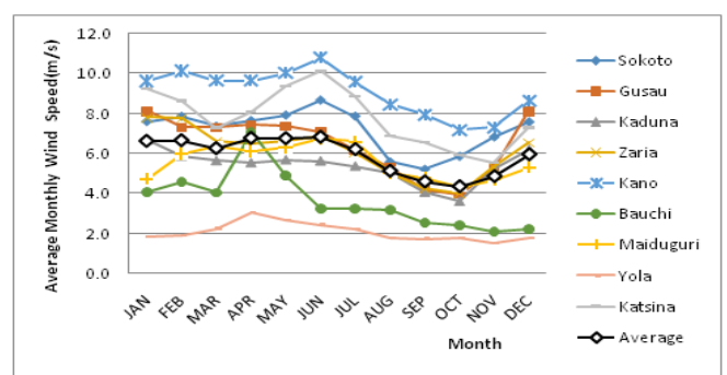
Fig 5d: Seasonal variation of Average Monthly wind speed (m/s) for Far-Northern cities against Months of the year.
