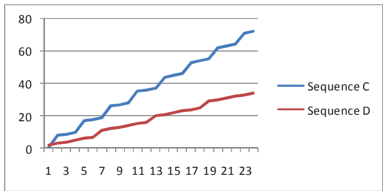
Figure 2 The line graph of sequences C and D. x axis = the number of terms y axis = the values of the terms in both sequences
