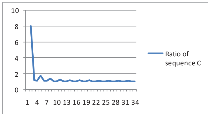
Figure 3 The ratio of sequence C x axis = terms of the sequence y axis = ratio of 2 consecutive numbers of sequence C
