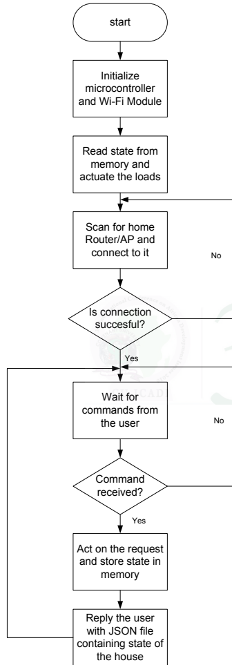
Fig. 6 Program Flow Chart
