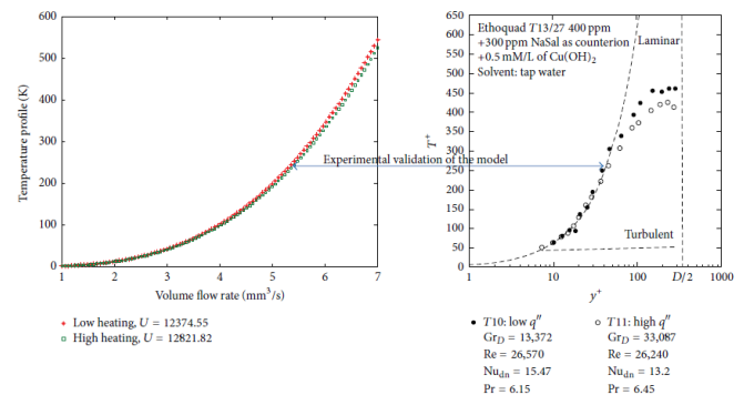
Figure 1: Theoretical Model using the unified number in laminar flow and was validated via experiments of two turbulent flow (Gasljevic et al., 2000)Ref (6)
