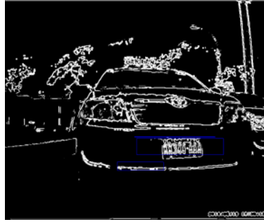
Fig.8: Localization of license plate
