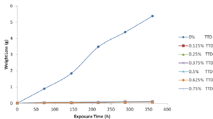
Figure 2. Variation of weight-loss with exposure time for samples (A – G) in 3 M \text{H}_2\text{SO}_4 .
