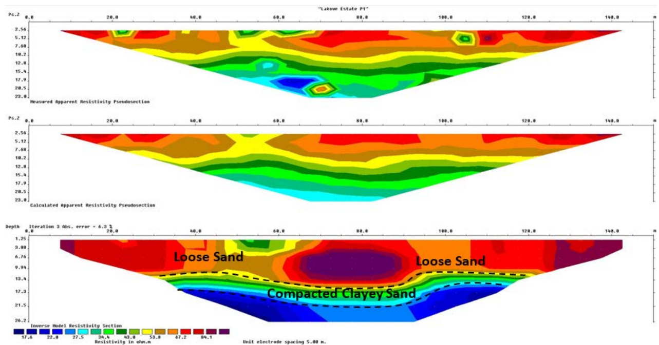
Figure 5: Inverse resistivity model of traverse P1
